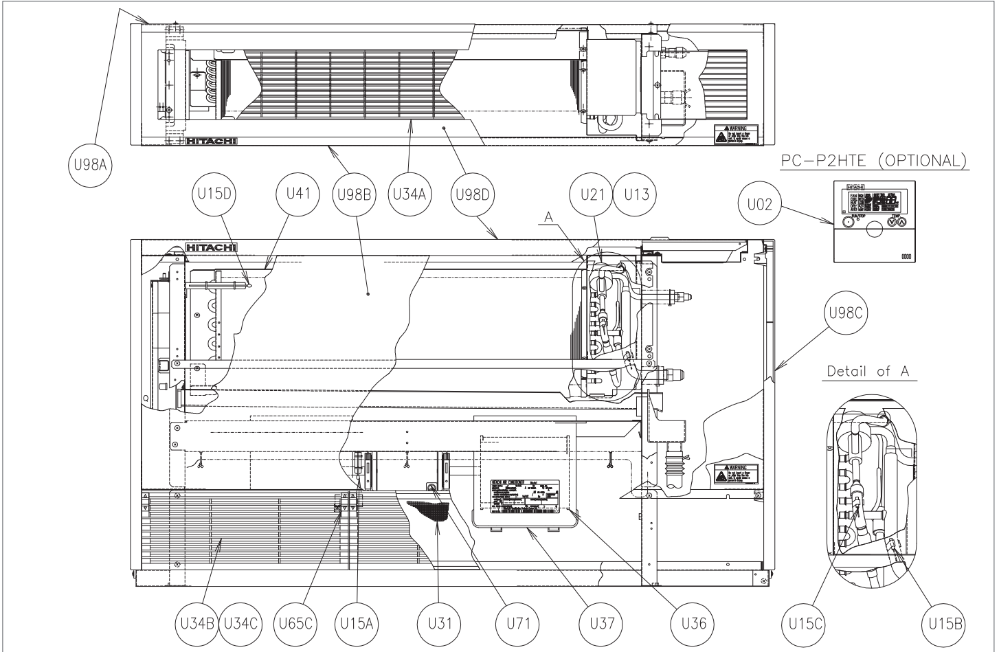
LOCATION OF ELECTRICAL EQUIPMENT IN THE ELECTRICAL CONTROL BOX
