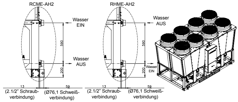
Detail A
